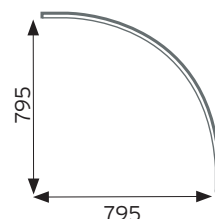
90° inner curve 1300 mm Graphic on inner radius 0,8 m.
